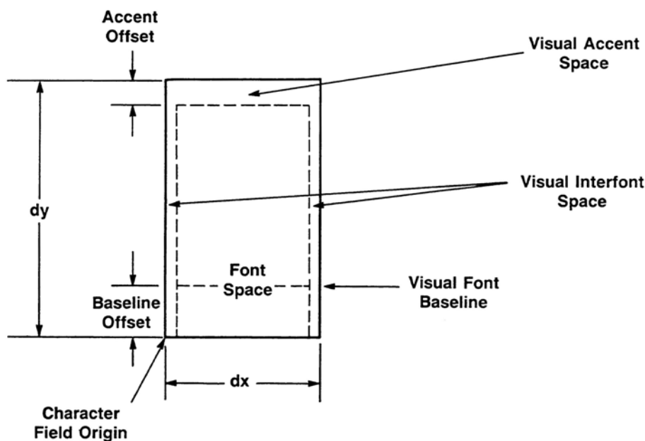
Figure D1 Character Field Layout
